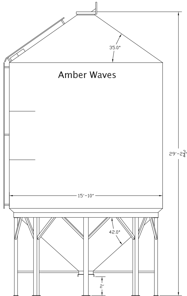
MODEL 1630 SIDE VIEW
