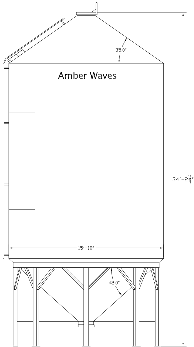
MODEL 1640 SIDE VIEW
